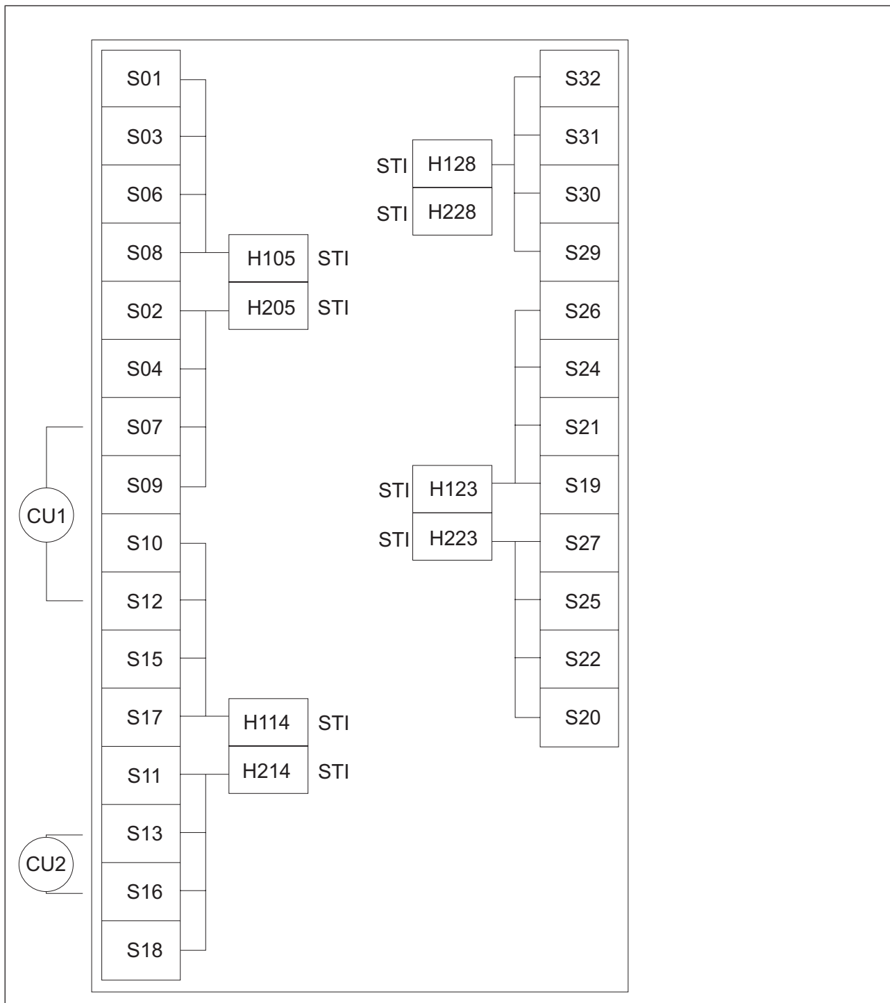
Figure 6. I/O channel path configuration for a representative I/O cage in a 2094 or 2096 model
