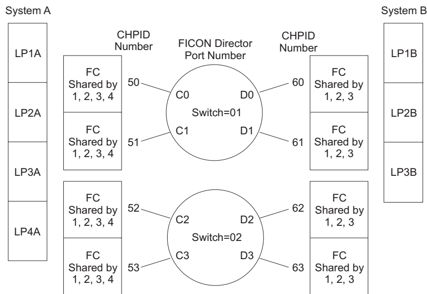
Figure 50. FICON CTC (fully redundant)
