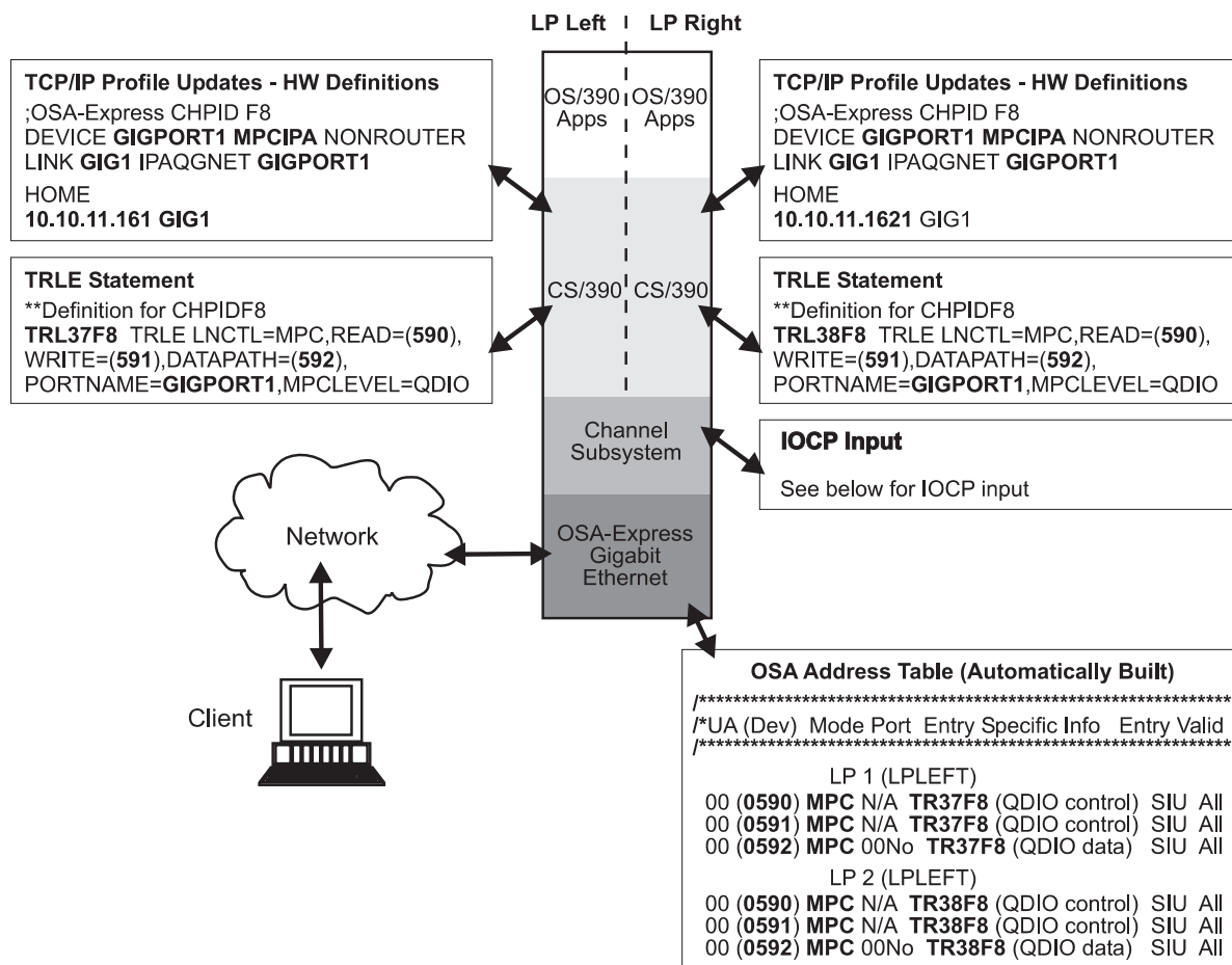
Figure 44. OSA configuration with two logical partitions
