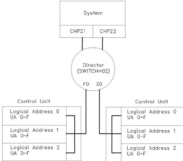
Figure 40. Control unit logical addressing
