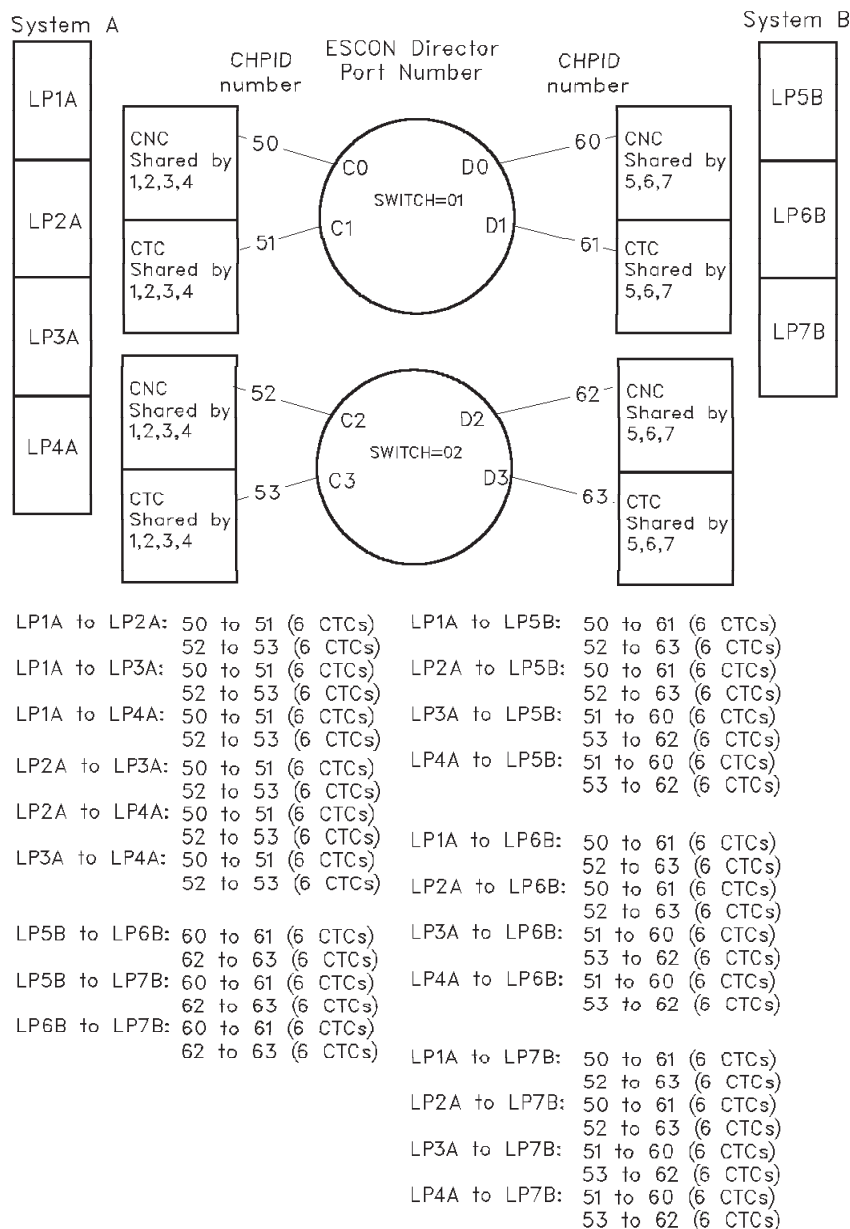
Figure 49. ESCON CTC with shared channels
