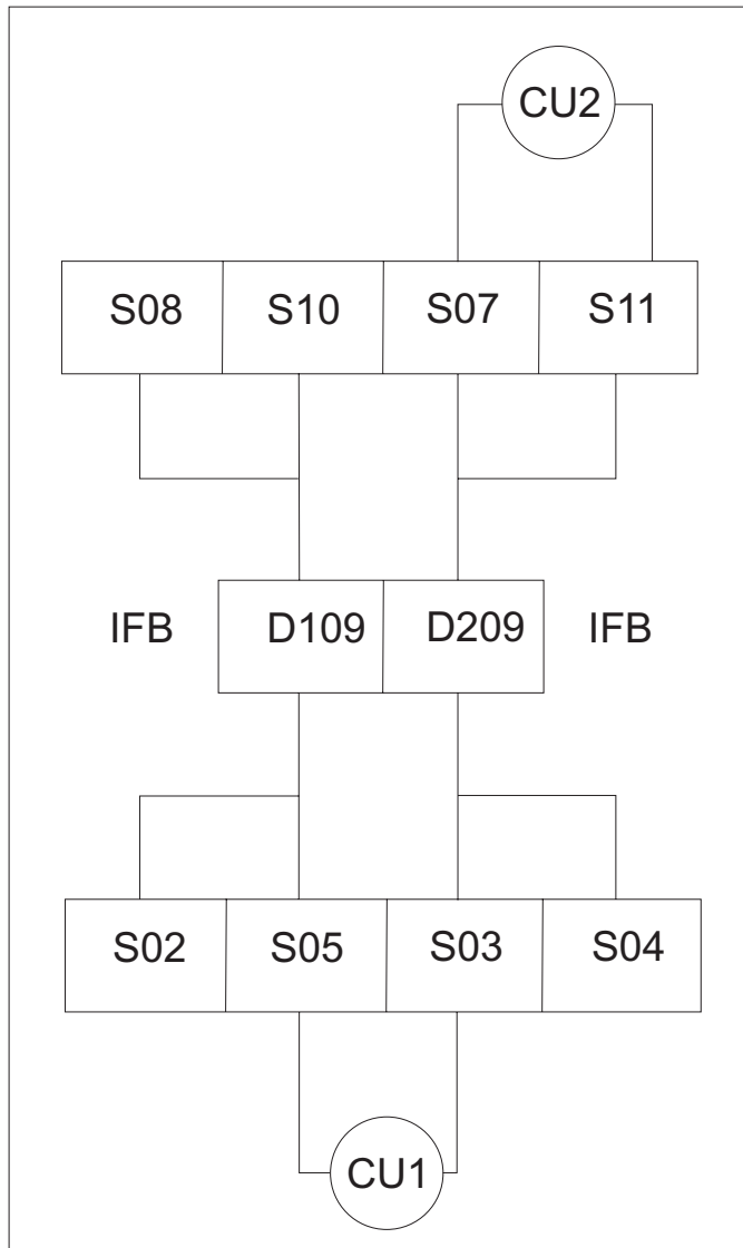
Figure 5. I/O channel path configuration for a representative I/O drawer in a 2098 model
