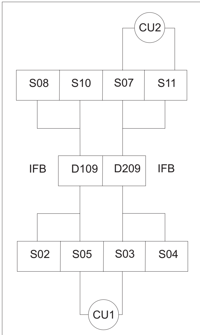
| Figure 3. I/O channel path configuration for a representative I/O drawer in a 2817, 2818 and 2827 model
