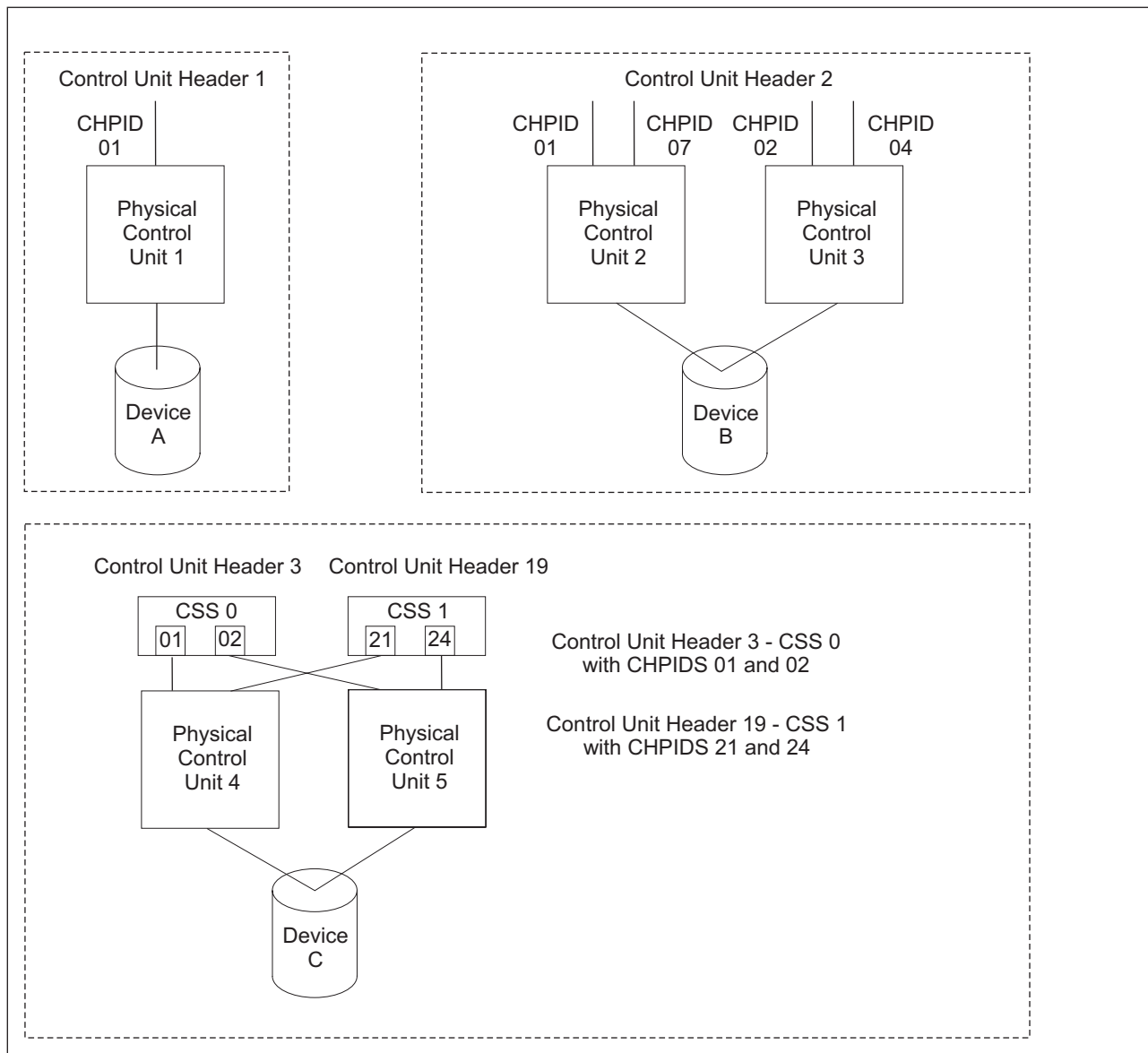
Figure 10. Valid control unit headers
