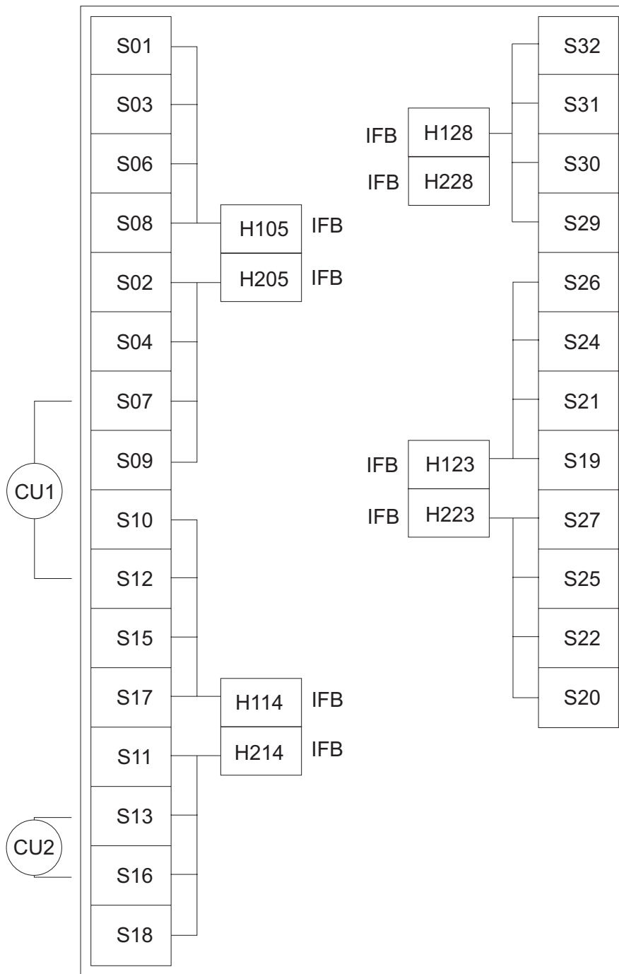
Figure 4. I/O channel path configuration for a representative I/O cage in a 2097 model
