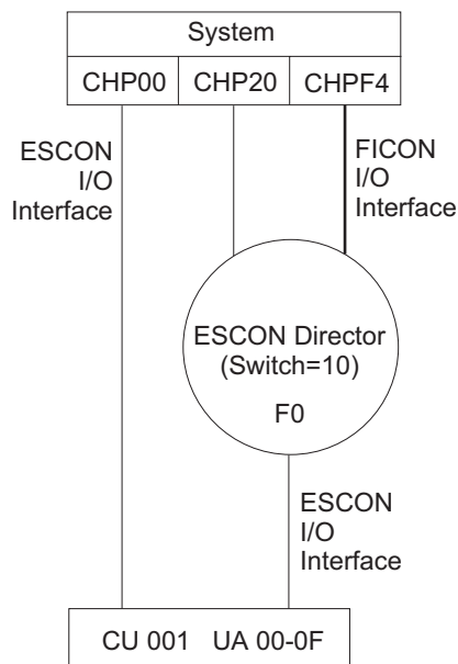
Figure 42. FCV channel configuration
