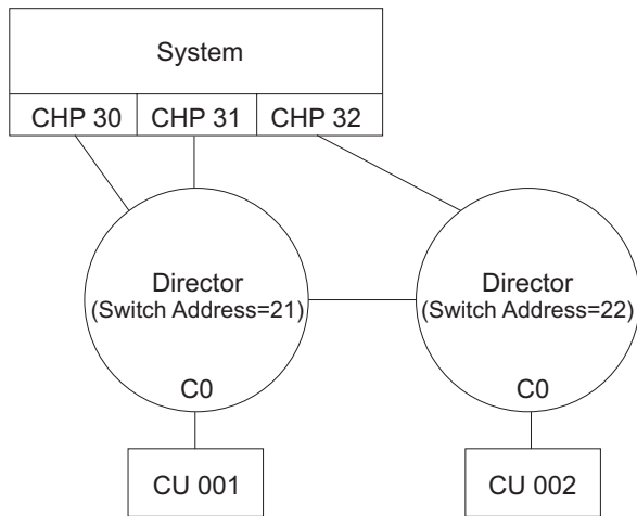
Figure 39. Cascaded FICON directors
