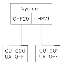
Figure 43. ESCON control units requiring unit address 00
