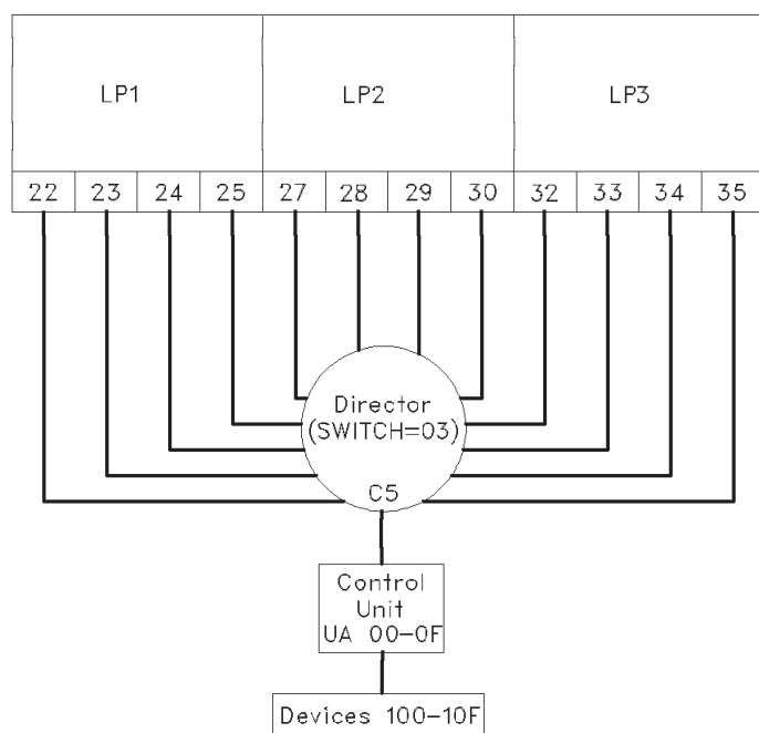
Figure 33. LPAR mode with more than eight paths to an ESCON device
