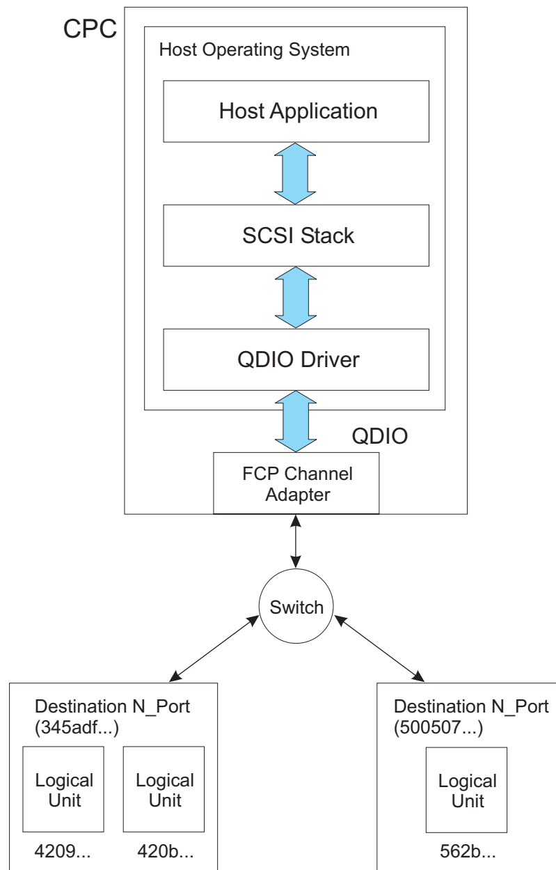
Figure 46. FCP channel configuration
