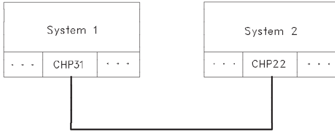
Figure 35. ESCON CTC point-to-point
