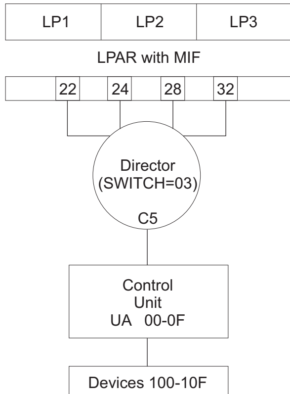
Figure 34. LPAR mode with shared paths to an ESCON device
