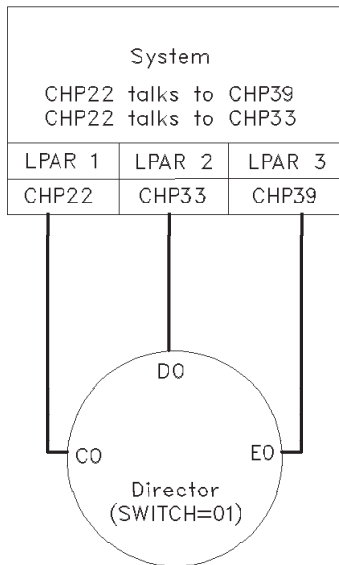
Figure 36. ESCON CTC dynamic through an ESCON director with multiple paths
