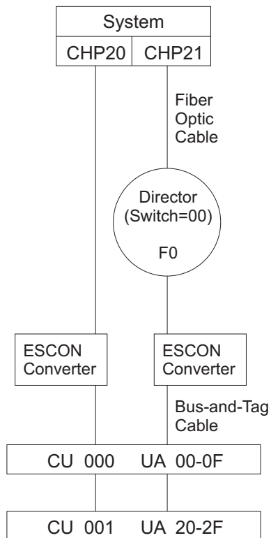
Figure 41. Channels through an ESCON converter
