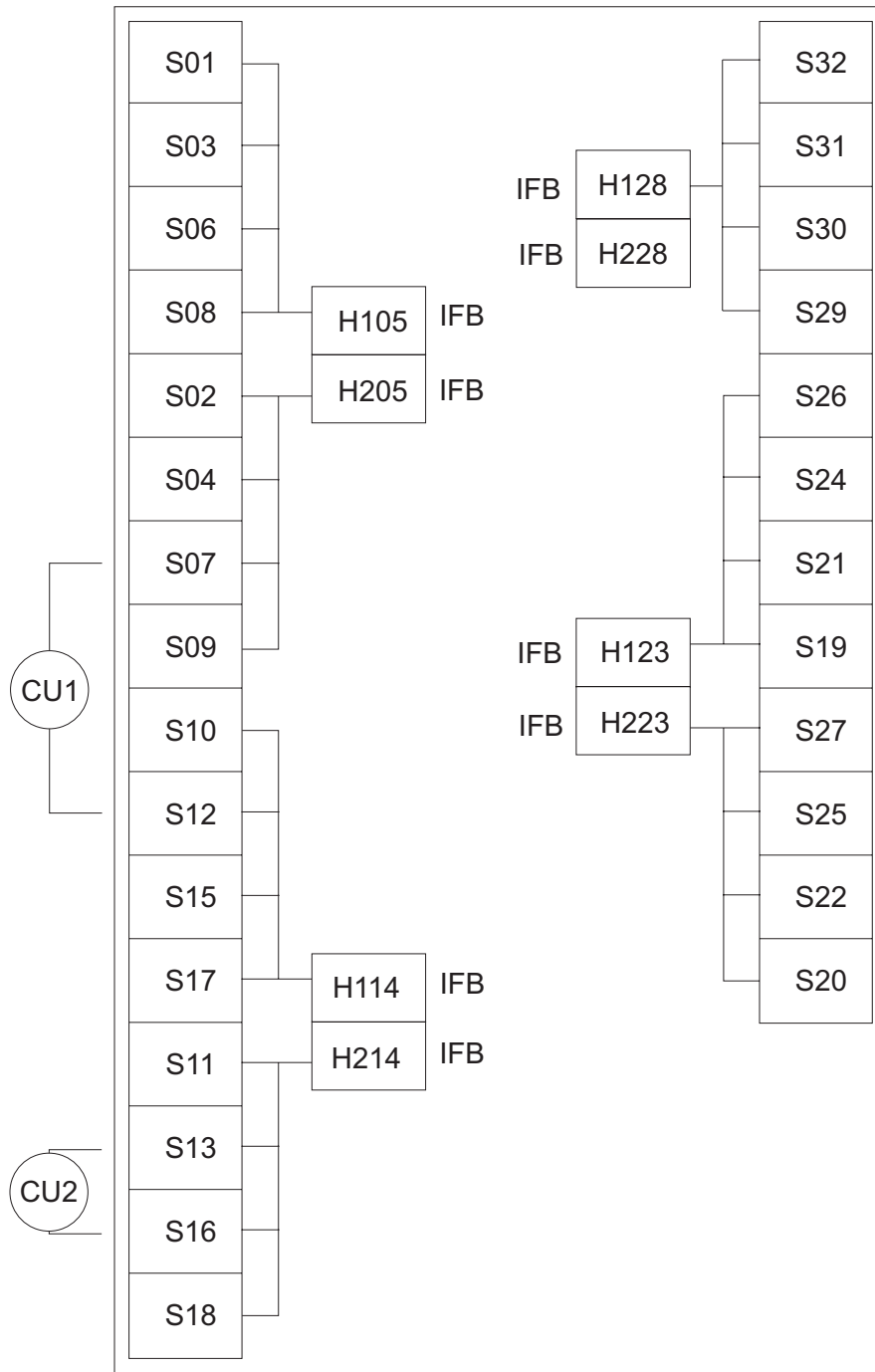
Figure 2. I/O channel path configuration for a representative I/O cage in a 2827 and 2817 model
