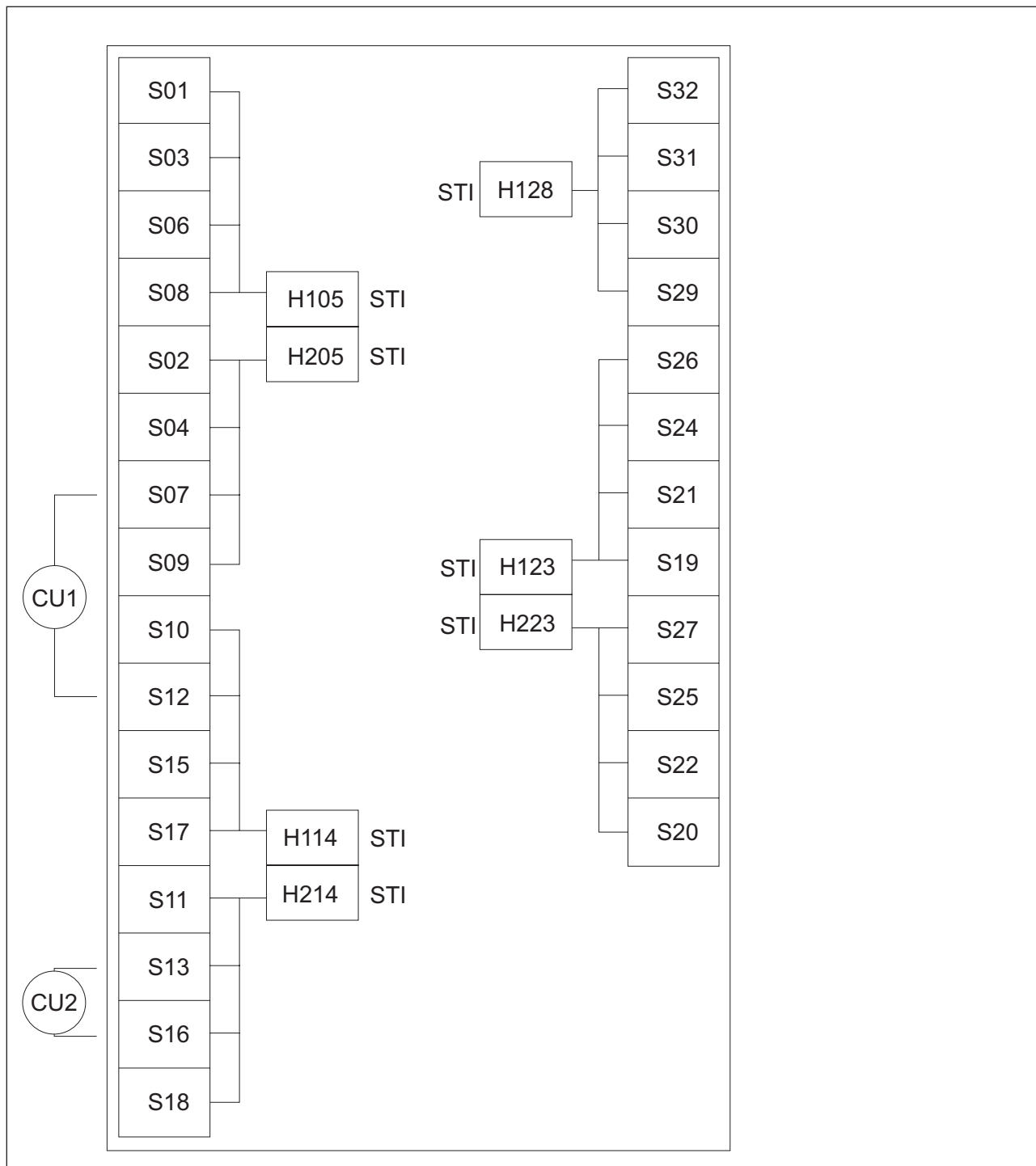
Figure 7. I/O channel path configuration for a representative I/O cage in a 2084 or 2086 model
