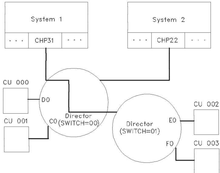
Figure 38. Chained ESCON directors
